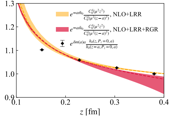
FIG. 11: The ratio of P_z = 0 matrix elements (black points) defined in Eq. (28) are shown. The bands are inferred from the NLO+LRR and NLO+LRR+RGR Wilson coefficients respectively with scale variation.
