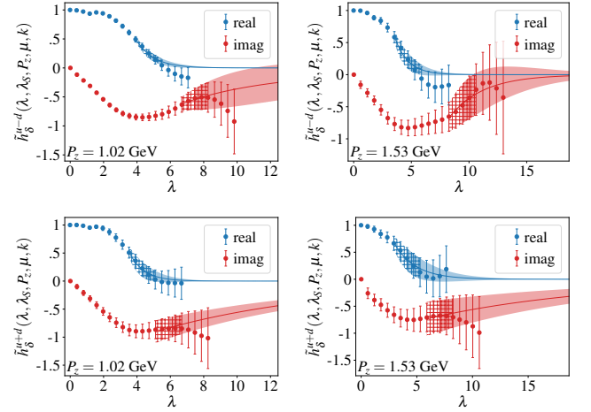
FIG. 13: The (upper) isovector and (lower) isoscalar hybrid renormalized matrix elements with (left) P_z = 4\frac{2\pi}{L} and (right) P_z = 6\frac{2\pi}{L} . The hatches show the range of data used for the fit to the extrapolation model and the bands are the result of that fit starting from \lambda_L . The hybrid renormalized data makes use of the NLO+LRR+RG Wilson coefficients computed at \mu_0 = 2e^{-\gamma_E}/z (i.e. k = 1 ) and subsequently evolved to \mu = 2 GeV.
