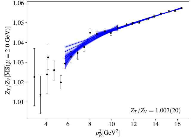
FIG. 17: Ratio of the tensor to vector current renormalization factors Z_T/Z_V as a function of the RI-MOM momentum p_R . The conversion from RI-MOM to \overline{\text{MS}} is done at four loops. The bands show the 18 different fits considered, all overlaid on top of one another. The AIC-averaged result final result for the ratio is given in the bottom right corner.
