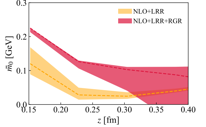
FIG. 10: The \bar{m}_0 determined using NLO+LRR and NLO+LRR+RGR Wilson coefficients are shown. The bands come from the scale variation.
